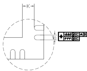
DETAIL : "A" (2/1)
