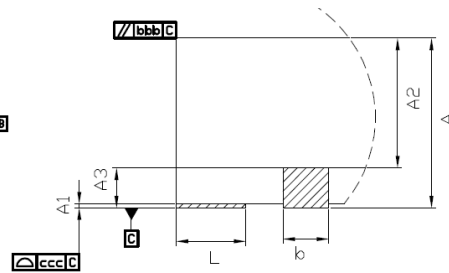
DETAIL : "B" (5/1)
