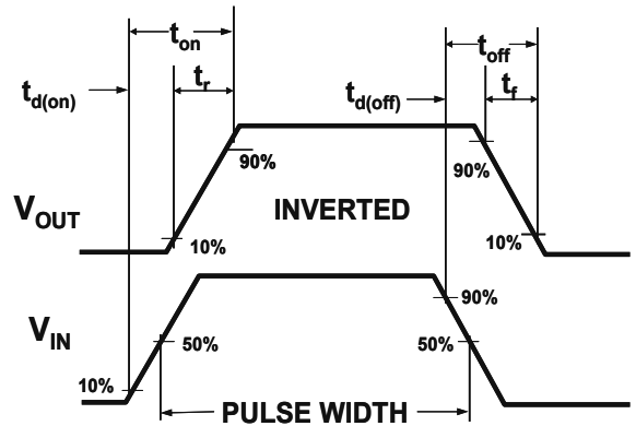
Figure 2: Switching Waveforms
