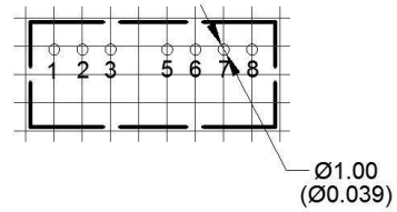
Printed board vertical view
