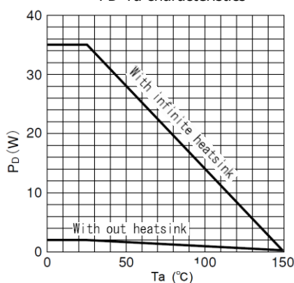
PD-Ta characteristics
