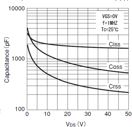
Capacitance- 5 VDS characteristics (typical)
