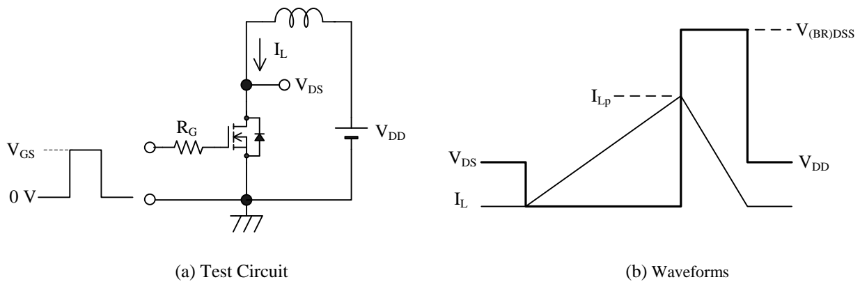
Figure 1 Unclamped Inductive
