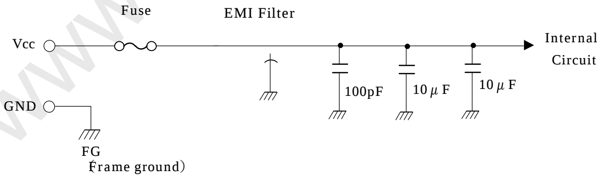
Figure 8-2(A) Equivalent circuit of logic signal Input
