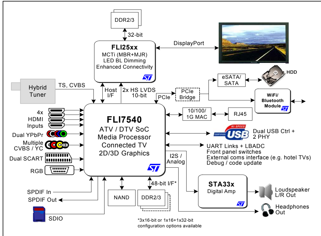
Figure 1. EU/US DTT + cable iDTV application
