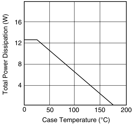
www.DataSheet4U.com POWER DERATING CURVE
