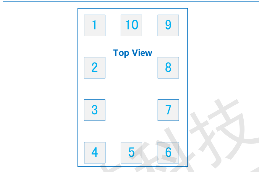
Figure 2. FM1694 Pinout - 10-Pin QFN (Top View)
