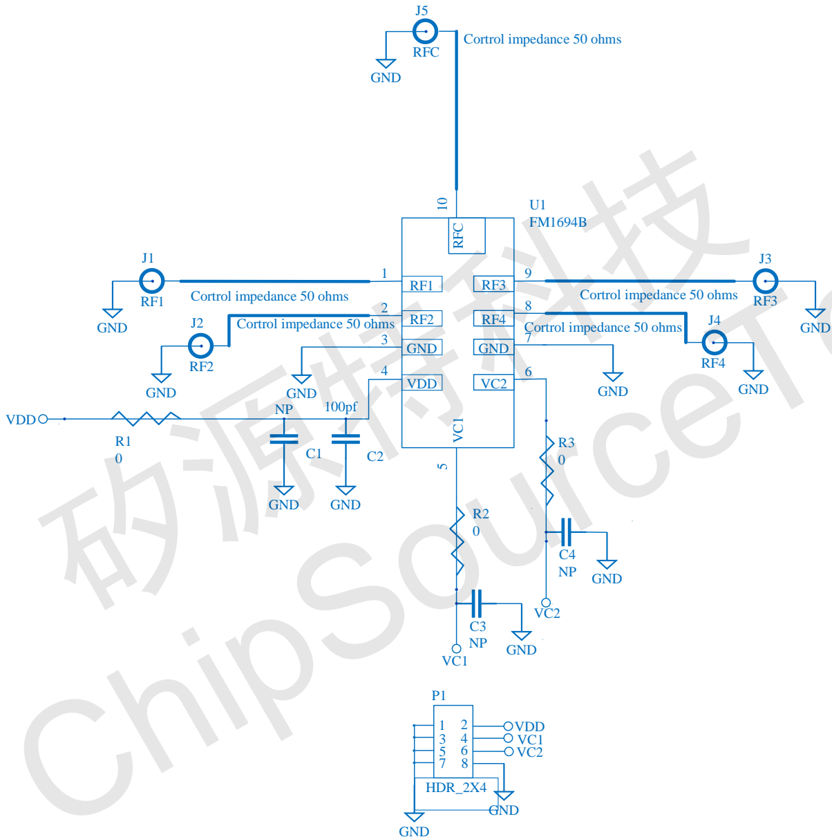
Figure 3. FM1694 Application Schematic
