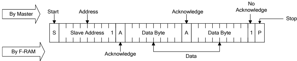
Figure 8. Sequential Read
