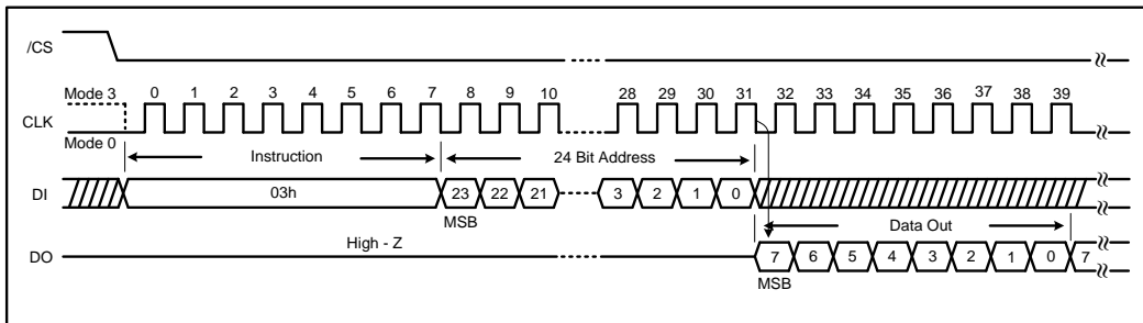
Figure 10. Read Data Register Instruction Sequence Diagram
