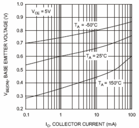
I_C , COLLECTOR CURRENT (mA) Fig. 4, Base Emitter Voltage vs. Collector Current (NPN5551)
