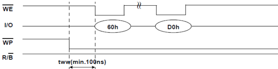
Figure 30 : t_{WW} in Erase Operation
