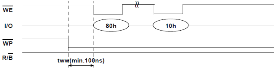
Figure 29 : t_{WW} in Program Operation
