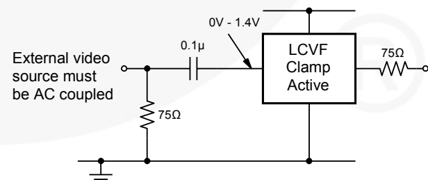
Figure 16. SCART with DC-Coupled Outputs
