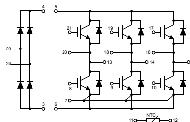
Internal Circuit Diagram
