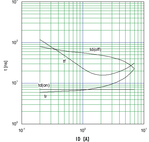
Typical Switching Characteristics vs. I D t=f(I_D):V_{cc}=300V, V_{GS}=10V, R_G=27\text{ }\Omega
