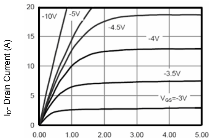
Figure 5 Output Characteristics
