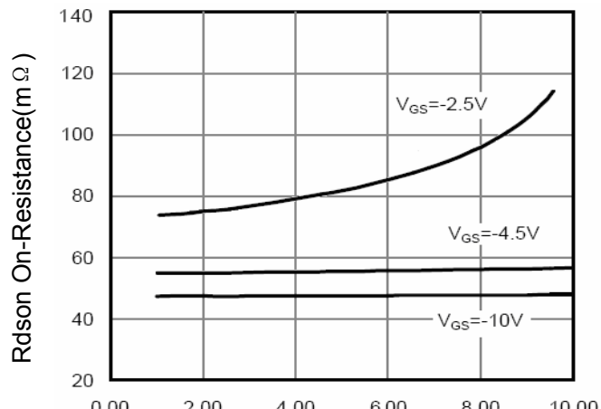
Figure 6 Drain-Source On-Resistance
