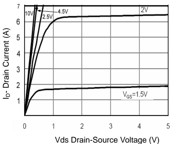
Figure 5 Output CHARACTERISTICS
