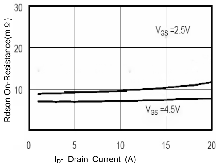
Figure 4 Drain-Source On-Resistance
