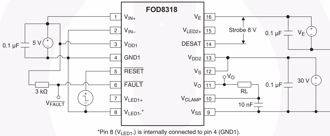
Figure 45. Reset Delay ( t_{RESET(FAULT)} ) Test Circuit
