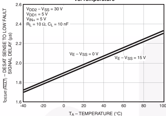
Figure 25. DESAT Sense to Low Fault Signal Delay ( t_{\text{DESAT(FAULT)}} ) vs. Temperature
