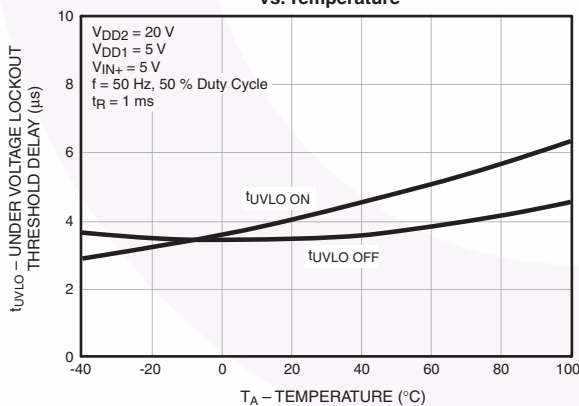
Figure 29. Under Voltage Lockout Threshold Delay ( t_{\text{UVLO}} ) vs. Temperature
