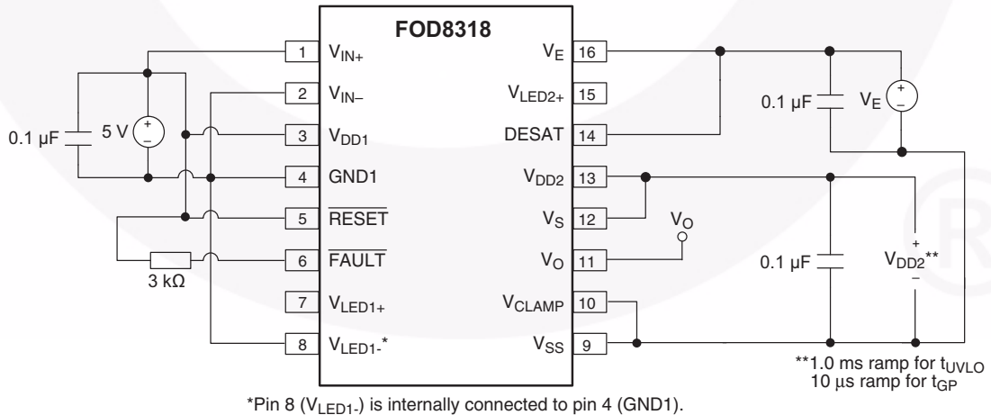
Figure 46. Under-Voltage Lockout Delay ( t_{UVLO} ) and Time to Good Power ( t_{GP} ) Test Circuit
