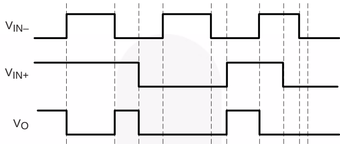
Figure 57. Input/Output Relationship
