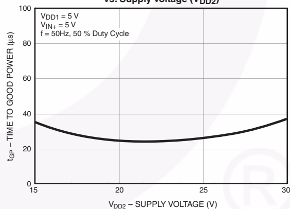
Figure 30. Time to Good Power ( t_{\text{GP}} ) vs. Supply Voltage ( V_{DD2} )
