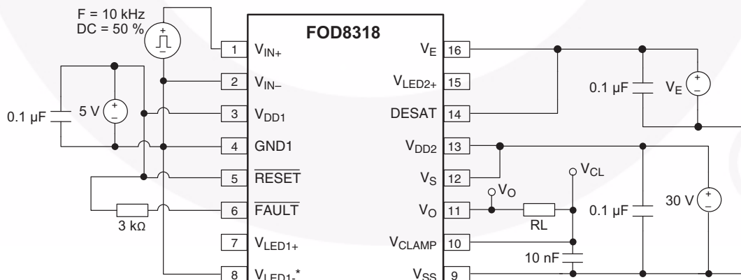
Figure 42. Under-Voltage Lockout Threshold ( V_{UVLO} ) Test Circuit
