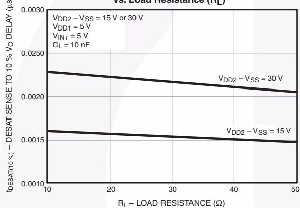
Figure 27. DESAT Sense to 10 % V_O Delay ( t_{\text{DESAT(10%)}} ) vs. Load Resistance ( R_L )
