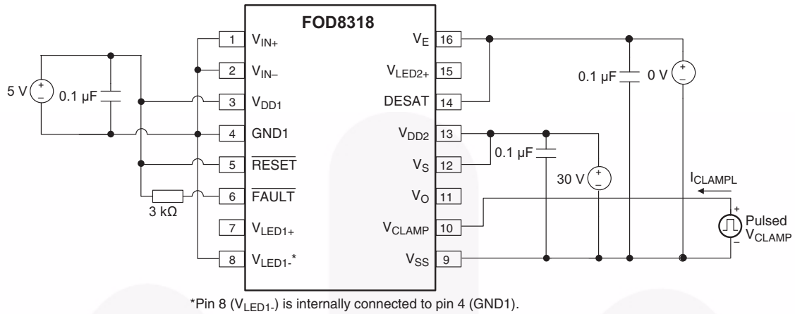
Figure 51. Clamp Low Level Sinking Current ( I_{CLAMP} )
