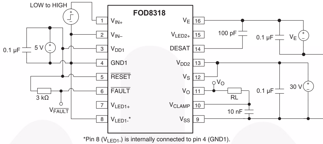
Figure 44. DESAT Sense ( t_{DESAT(90\%)} , t_{DESAT(10\%)} ), DESAT Fault ( t_{DESAT(FAULT)} ), and ( t_{DESAT(LOW)} ) Test Circuit
