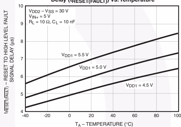
Figure 28. RESET to High Level FAULT Signal Delay ( t_{\text{RESET(FAULT)}} ) vs. Temperature
