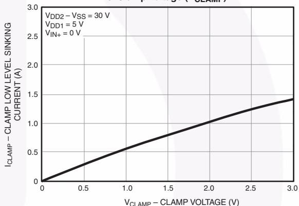
Figure 34. Clamp Low Level Sinking Current ( I_{CLAMPL} ) vs. Clamp Voltage ( V_{CLAMP} )
