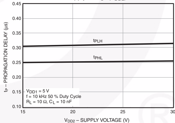
Figure 18. Propagation Delay ( t_p ) vs. Supply Voltage ( V_{DD2} )
