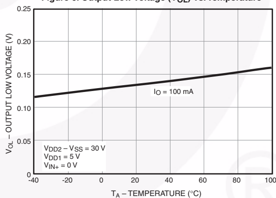
Figure 6. Output Low Voltage ( V_{\text{OL}} ) vs. Temperature
