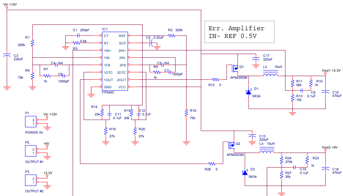
Figure 23. 2-channel dc-dc converter circuit
