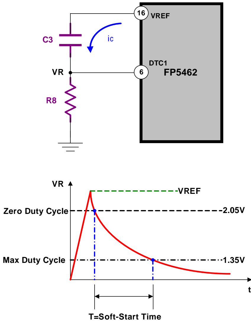
Figure 24 DTC Soft-start RC circuit and waveform
