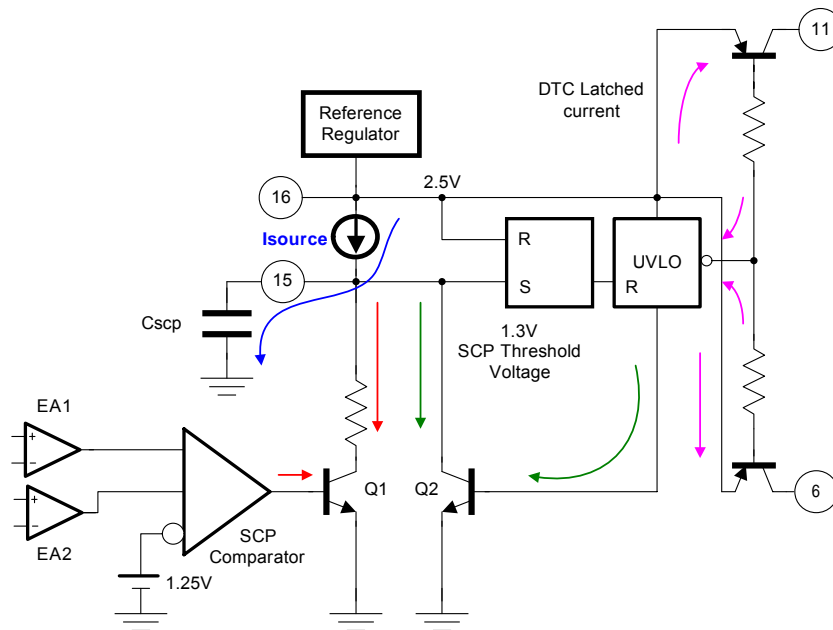
Figure 25 Internal SCP Detection/Control Circuits
