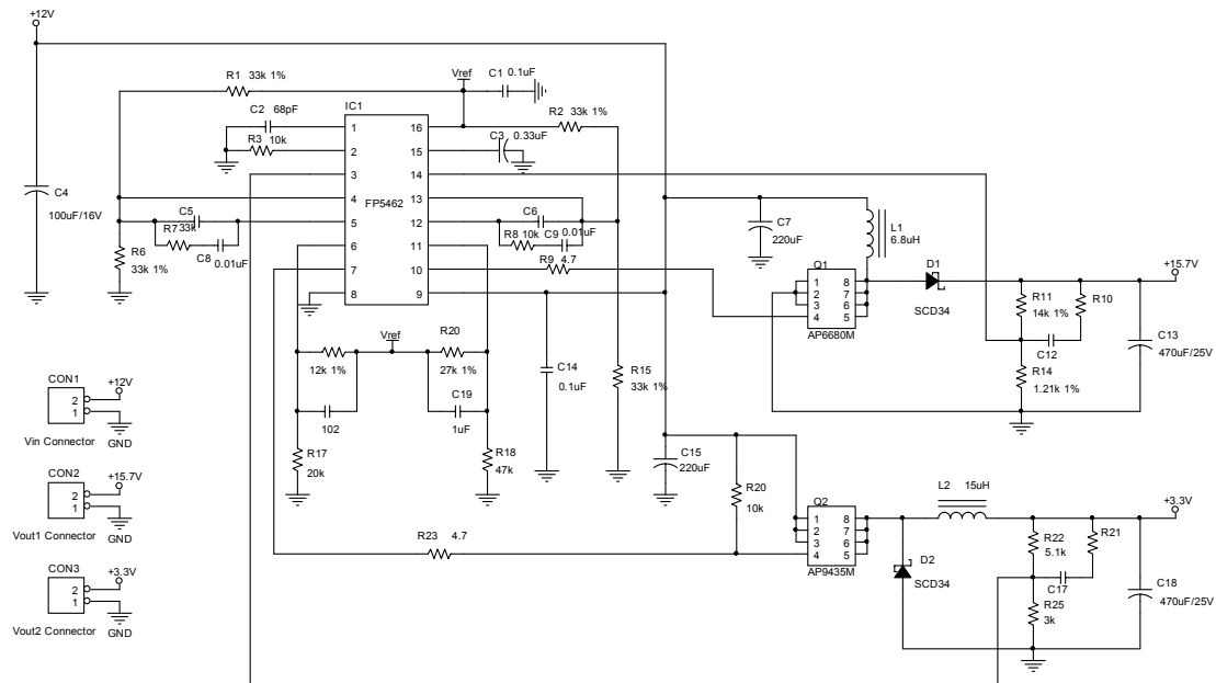
Figure 27 FP5462 Buck/Boost Regulators Application Circuits
