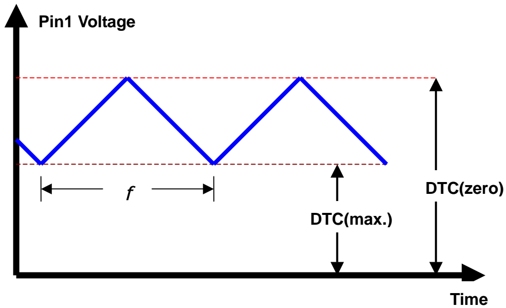
Figure 23 Oscillator Frequency with DTC voltage
