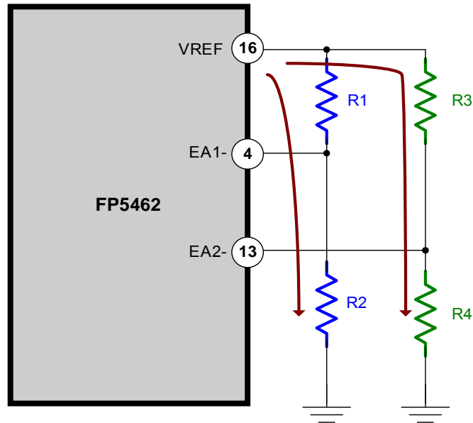
Figure 19 Reference and error amplifiers with resistive dividers
