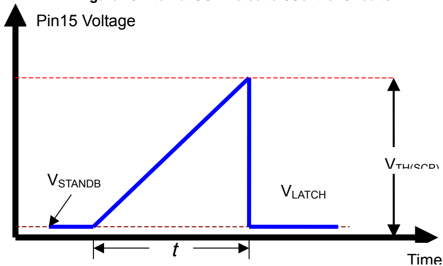
Figure 26 SCP waveform (SCP active)
