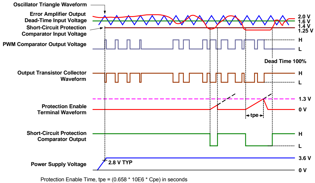
Figure 17 FP5462 CH1 Timing Diagram
