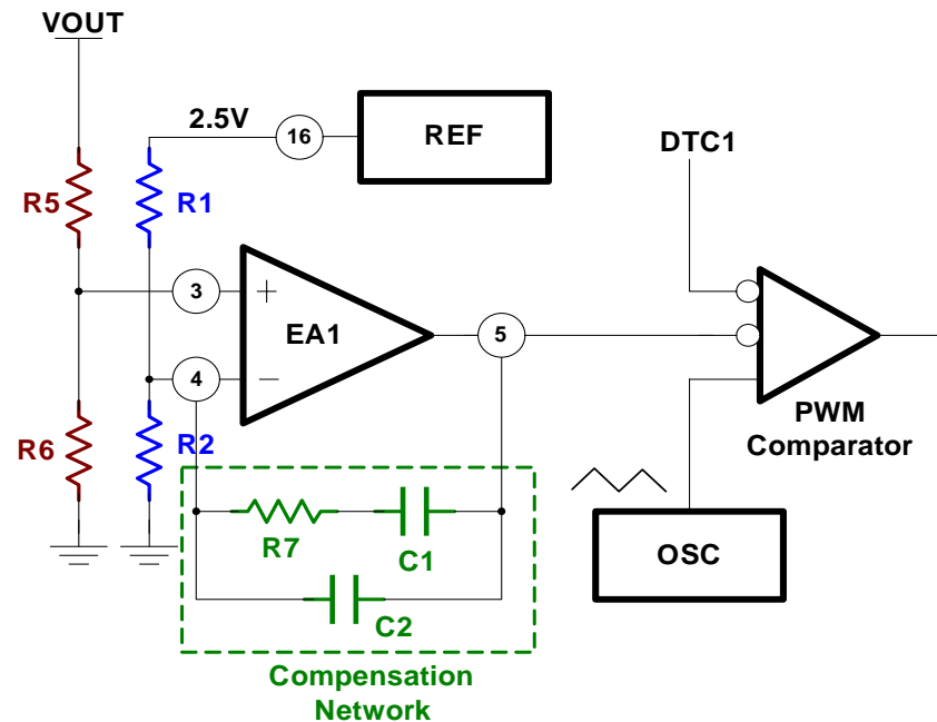
Figure 20 Error amplifier with Feedback/Compensation Circuits
