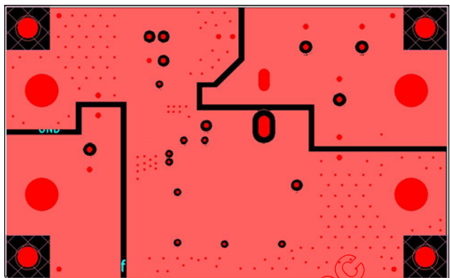
Figure 30. Inner layer 3
