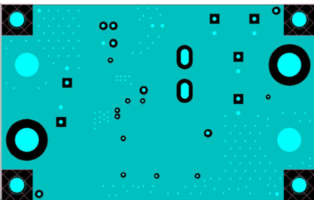
Figure 29. Inner Layer 2
