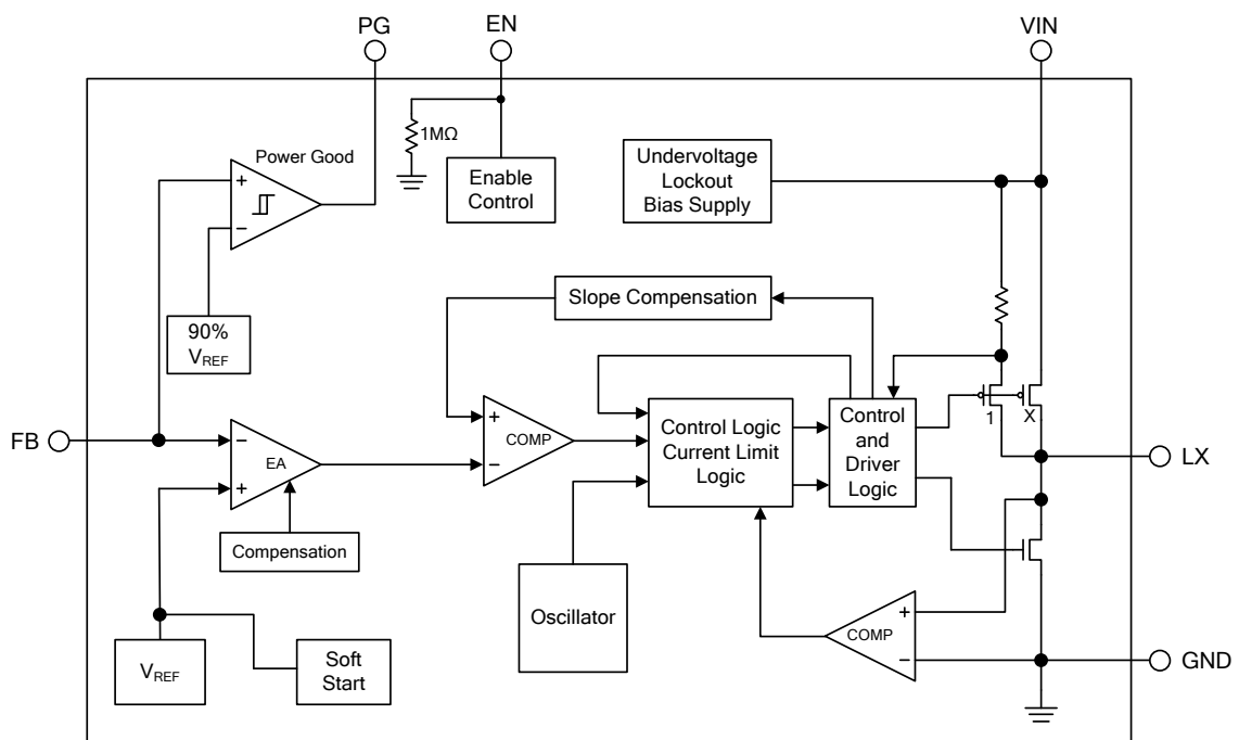
Figure 3. Block Diagram of FP6373
