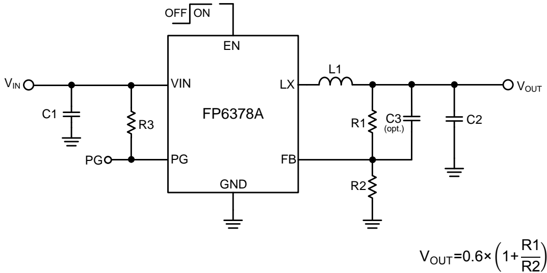
Figure 2. Schematic Diagram
