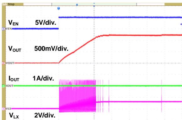
Figure 12. Power On through EN Waveform
