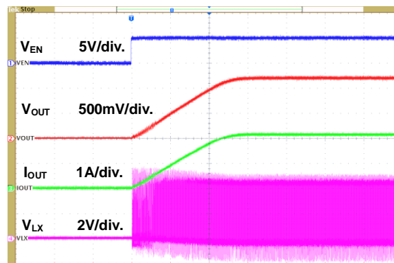
Figure 13. Power On through EN Waveform
