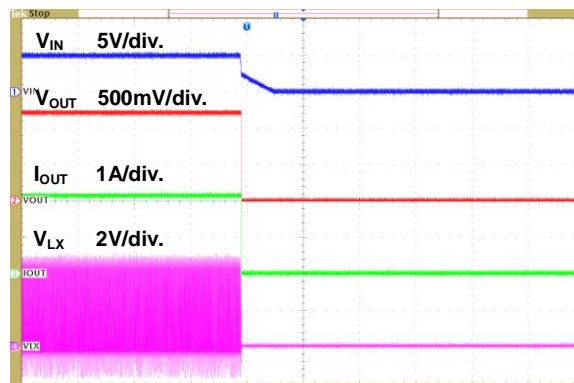
Figure 11. Power Off through VIN Waveform
