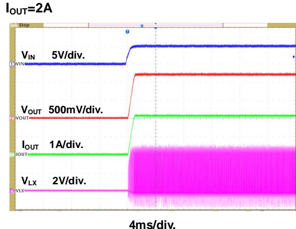
Figure 9. Power On through VIN Waveform
