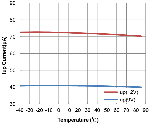
Figure 4. UP Current vs. Temperature
