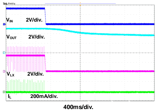
Figure 9. Power Off through VIN Waveform
