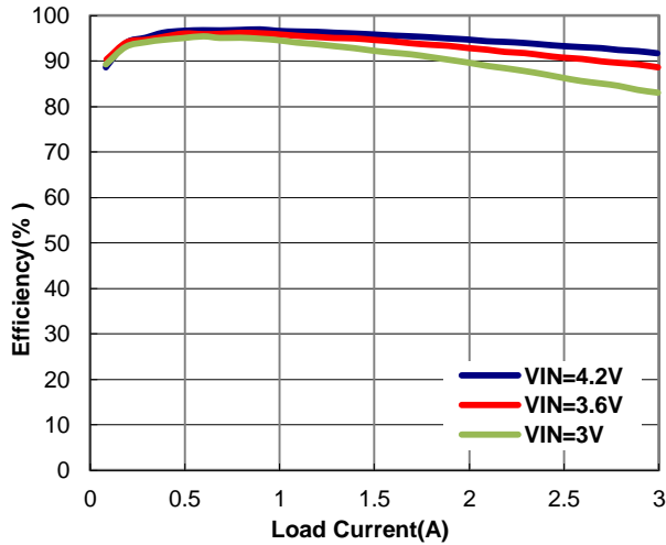
Figure 4. Efficiency vs. Output Current (VOUT=5V)
