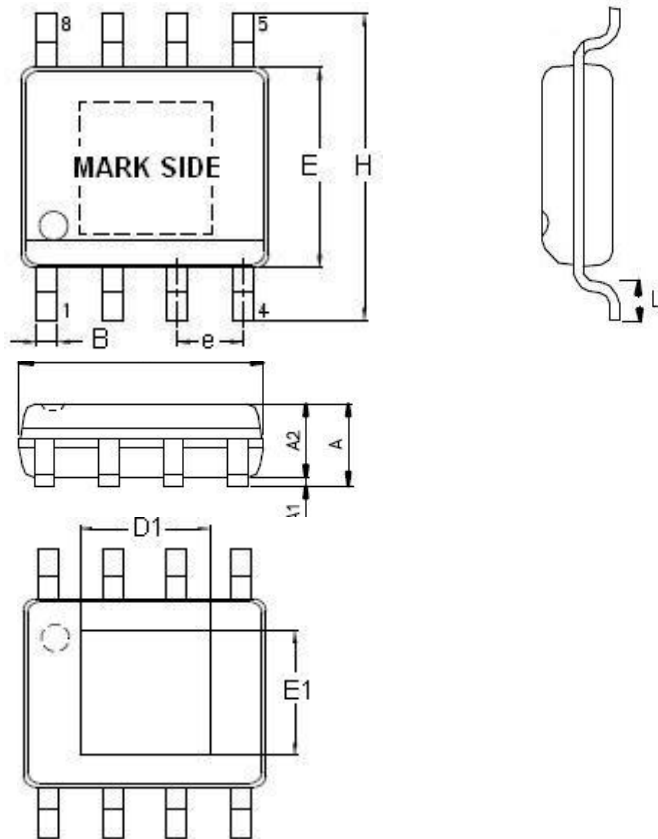
SOP-8 (Exposed Pad) Package (Unit: mm)
