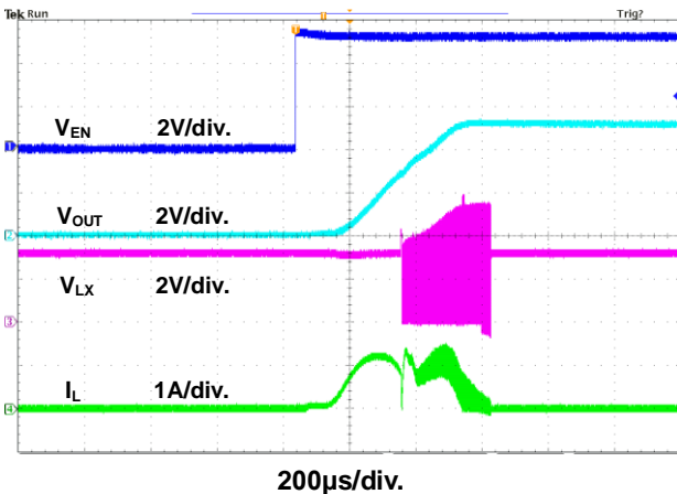
Figure 6. Power On through EN Waveform
