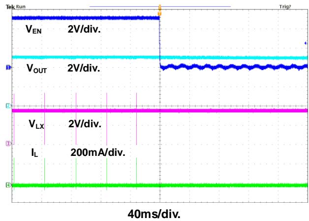
Figure 7. Power Off through EN Waveform
