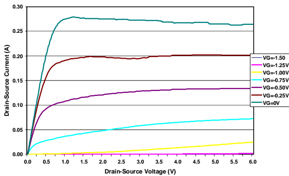
DC IV Curves FPD750SOT89
