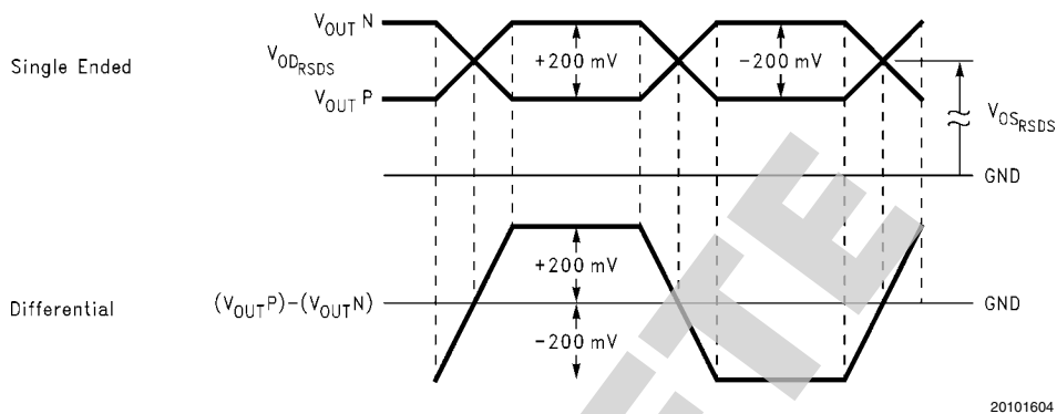
FIGURE 5. RSDS Waveform - Single Ended and Differential
