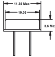
HC49S Resistance Weld
