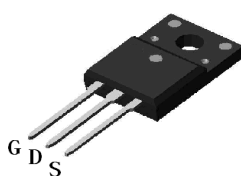
TO-220F
