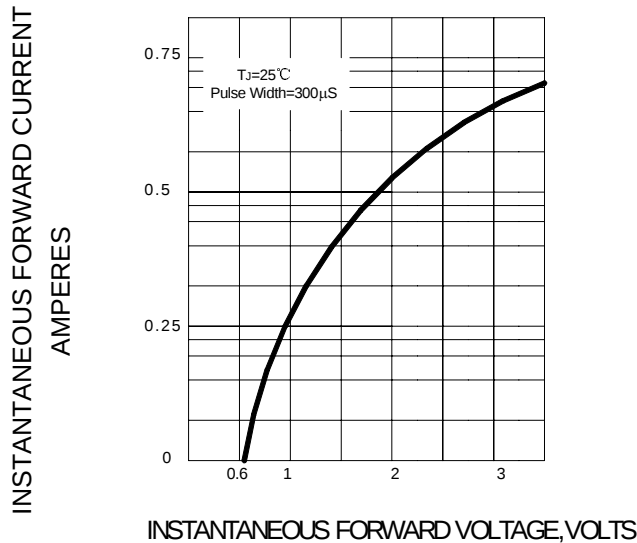
FIG.4-TYPICAL FORWARD CHARACTERISTIC
