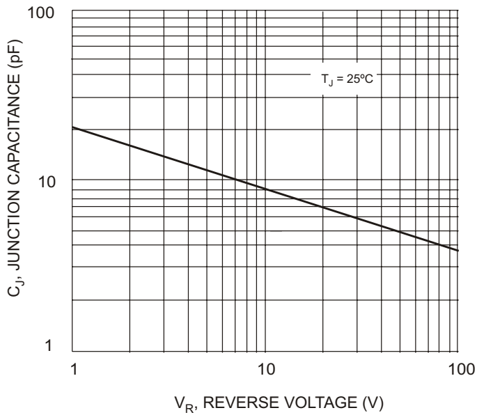
Fig. 3, Capacitance Characteristics
