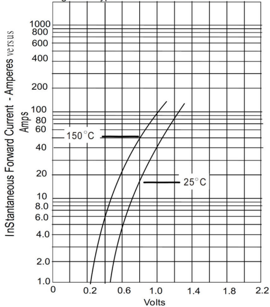
Figure .1-Typical Forward Characteristics
