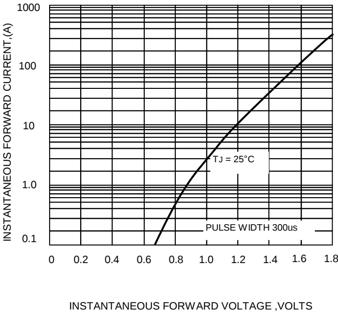
FIG.4-TYPICAL FORWARD CHARACTERISTICS
