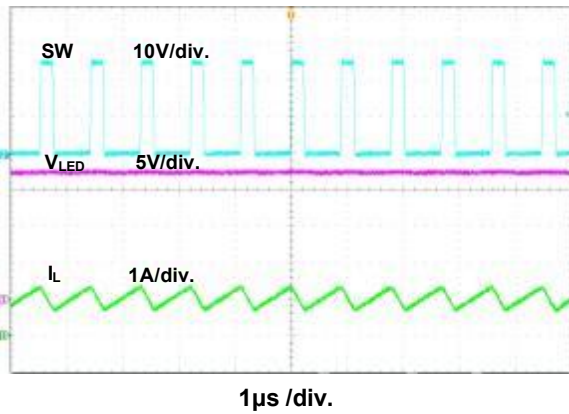
Figure 8. Switching Waveform
