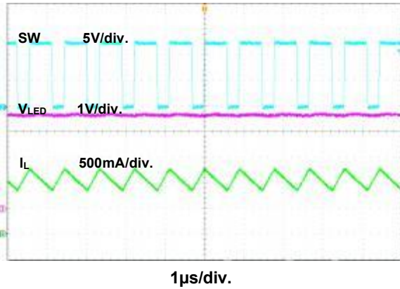
Figure 6. Switching Waveform
