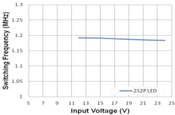
Figure 14. Frequency vs. Input Voltage (I OUT =0.5A)
