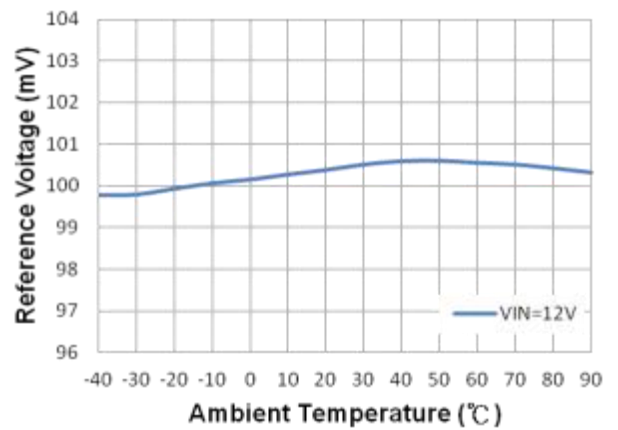
Figure 17. Reference Voltage vs. Temperature (I OUT =0.5A, 2S2P LED)
