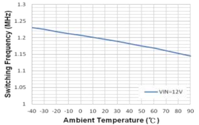
Figure 15. Frequency vs. Temperature (I OUT =0.5A, 2S2P LED)
