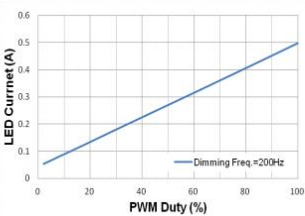
Figure 20. Digital Dimming :ILED vs. PWM Duty ( V_{in}=12V , 3S2P LED)
