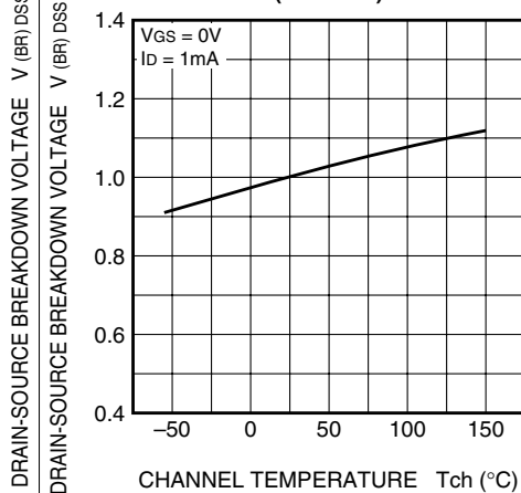
BREAKDOWN VOLTAGE VS. CHANNEL TEMPERATURE (TYPICAL)
