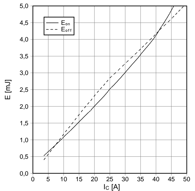
Schaltverluste IGBT-Wechselr. (typisch) switching losses IGBT-inverter (typical) E_{on} = f(I_c) , E_{off} = f(I_c) V_{GE} = \pm 15\text{ V} , R_{Gon} = 30\ \Omega , R_{Goff} = 30\ \Omega , V_{CE} = 600\text{ V} , T_{vj} = 125^\circ\text{C}
