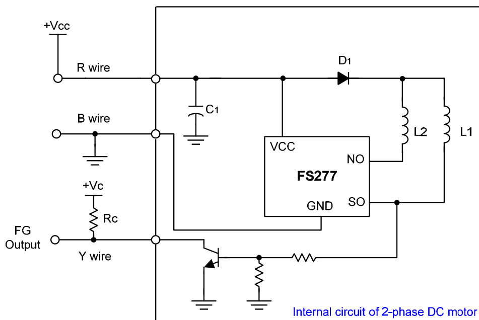
Fig 4 Application Circuit
