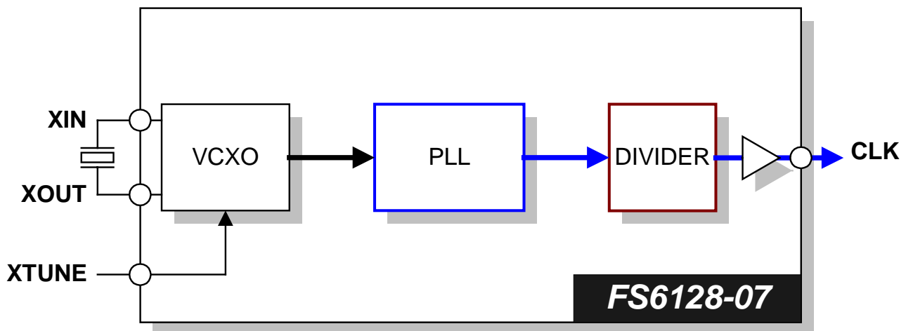
Figure 2: Block Diagram
