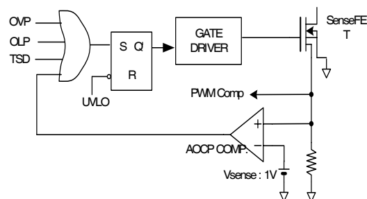
Figure 25. AOC block
