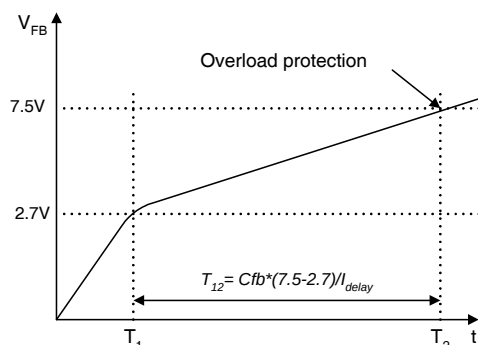
Figure 27. Overload protection
