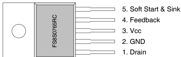
Figure 2. Pin Configuration (Top View)
