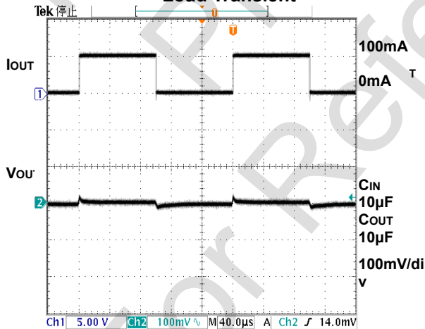
Load Transient
