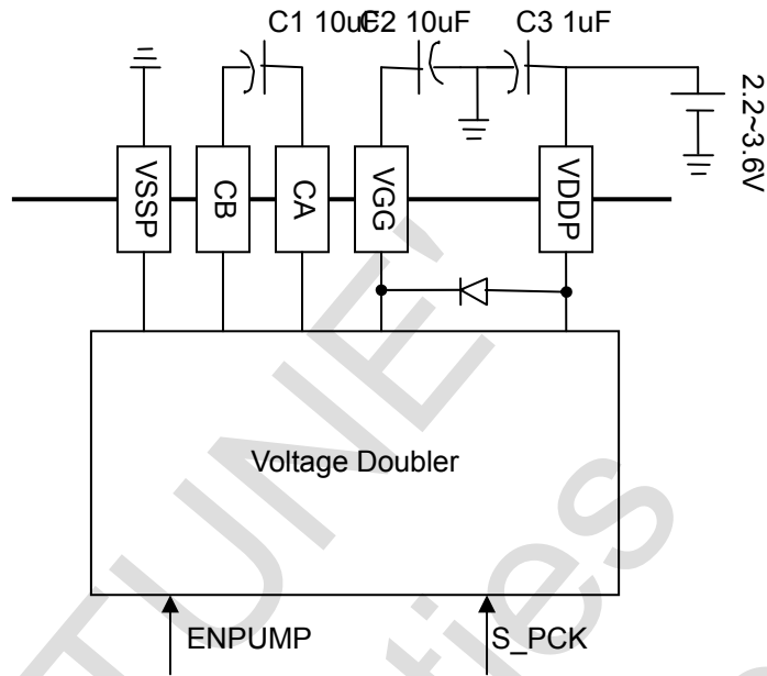
Figure 4-2 Voltage Doubler
