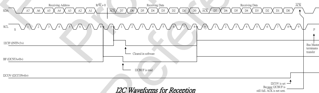
I2C Waveforms for Reception Figure 9-3 I2C waveform for reception
