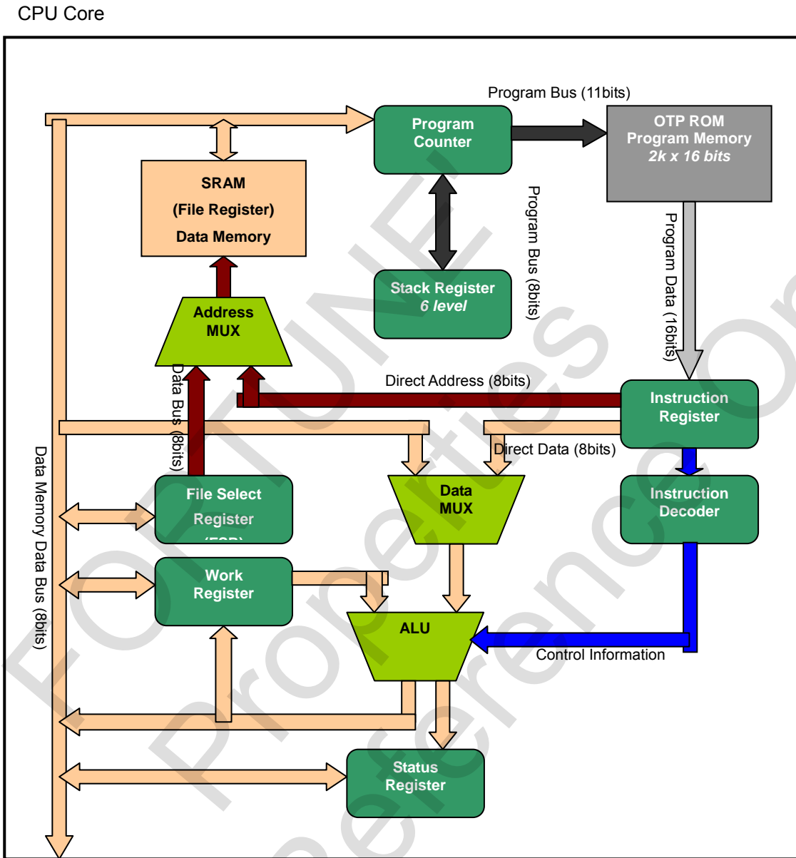
Figure 1-3 FS98021 CPU core function block
