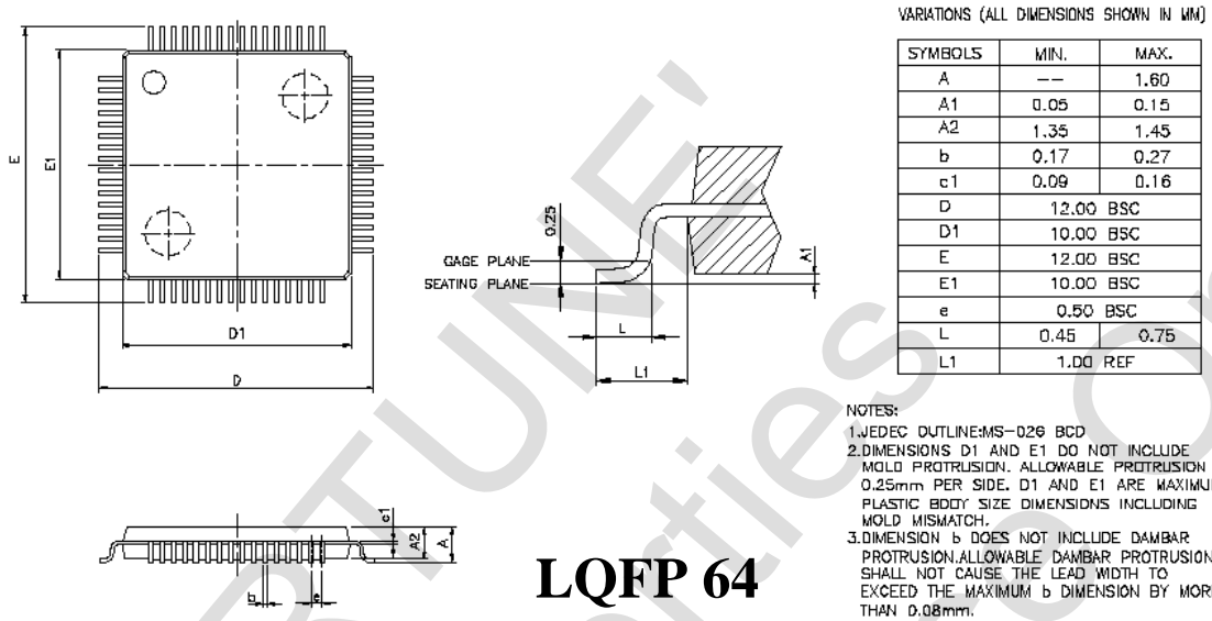
Figure 16-1 FS98021 package outline
