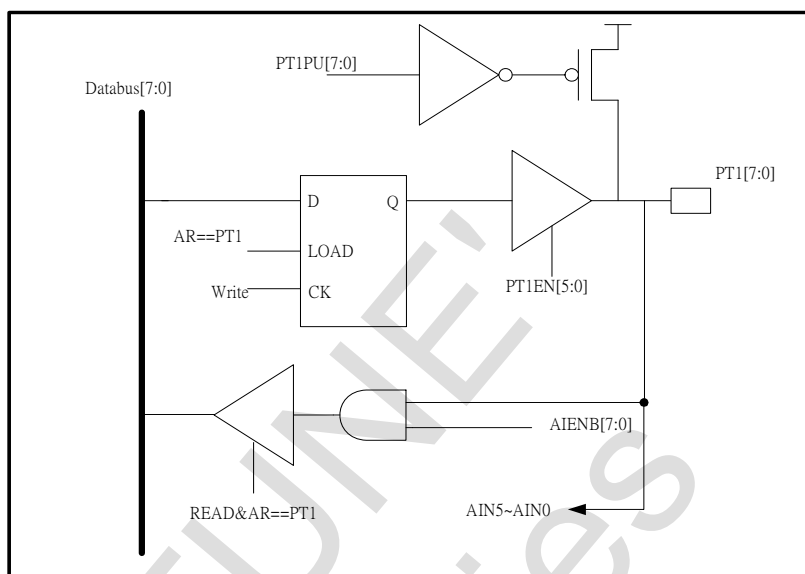
Figure 7-1 PT1[7:0] function block
