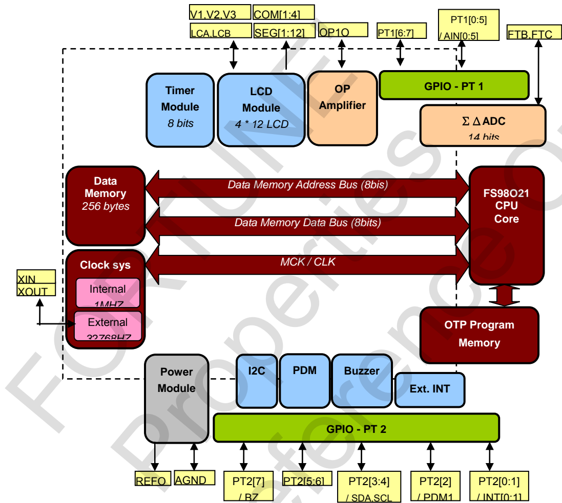
Figure 1-2 FS98021 function block
