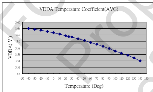
Figure 2-1 VDDA vs Temp @ VDD=3V
