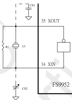
Diagram 9 Oscillation Circuit
