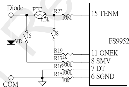
Diagram 29 Diode Measurement
