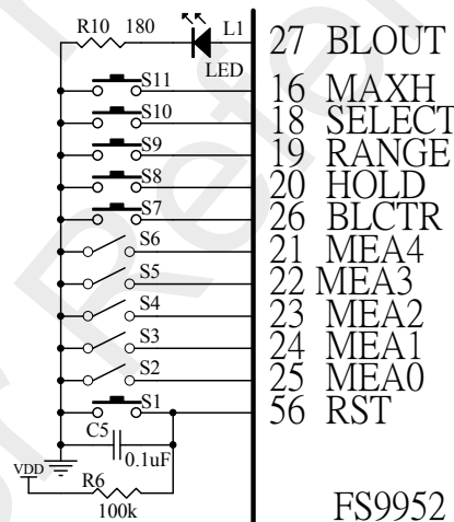
Diagram 10 Mode Switch and Function Control Circuit
