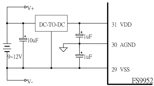
Diagram 21 9V~12V Power Supply
