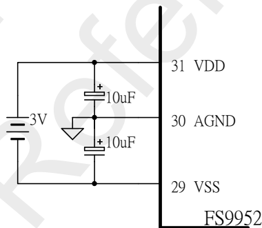
Diagram 16 3V Power Supply
