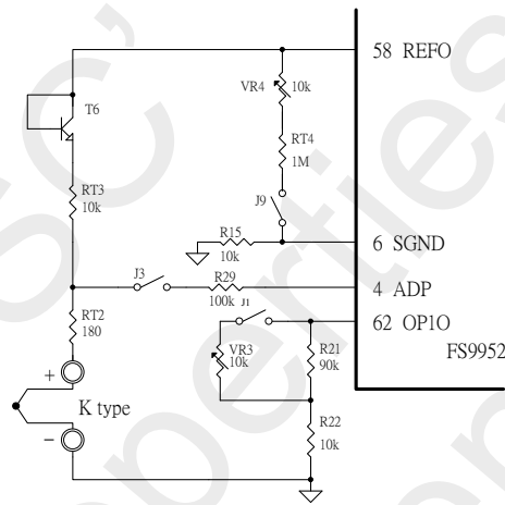
Diagram 34 Temperature Measurement (1)
