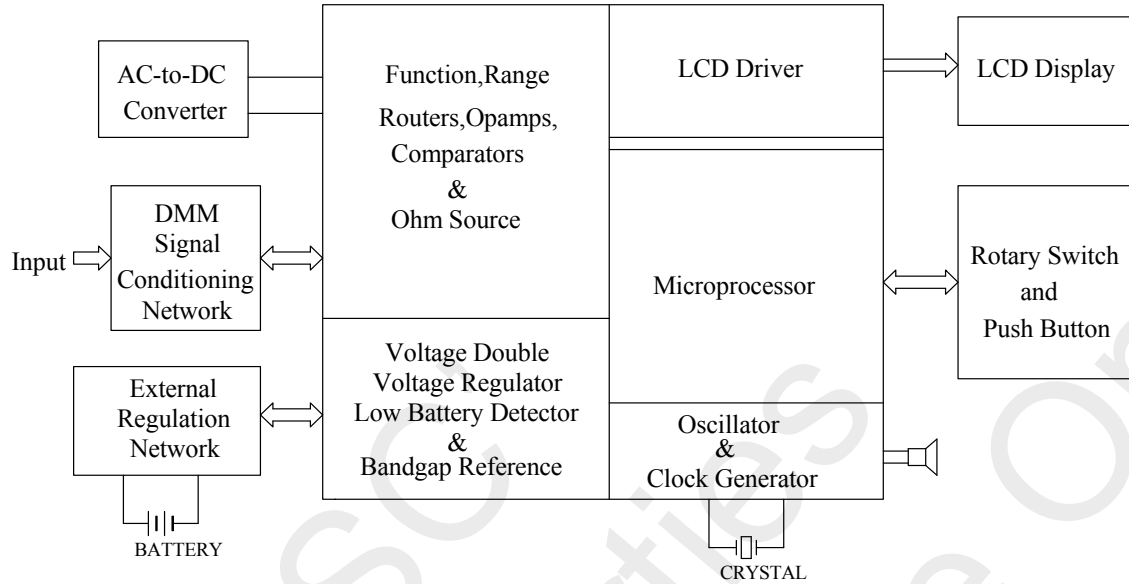
Diagram 1 Block Diagram
