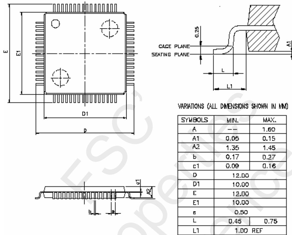
Package Outline
