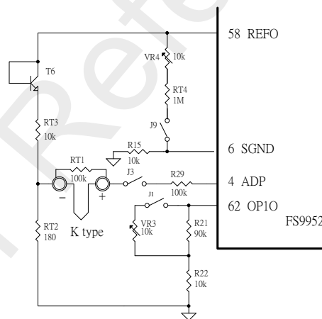
Diagram 35 Temperature Measurement (2)
