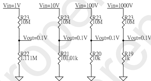
Diagram 26 Voltage Division Circuit Diagram
