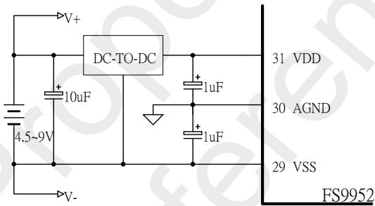
Diagram 19 4.5V~9V Power Supply
