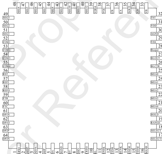
Diagram 2 64PIN Package
