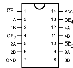
Pin Assignment for TSSOP
