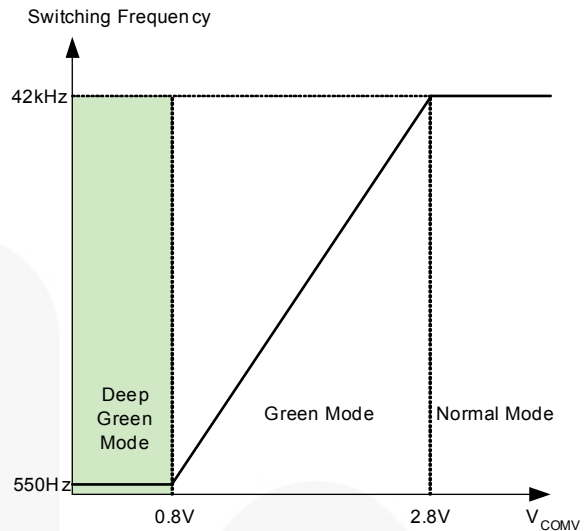
Figure 27. Switching Frequency in Green Mode
