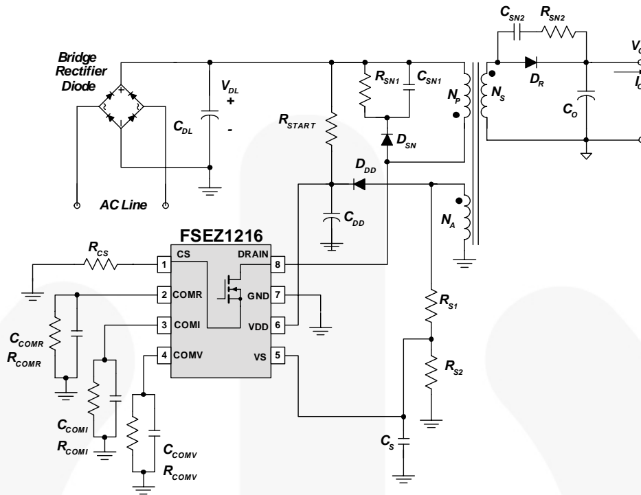
Figure 2. Typical Application
