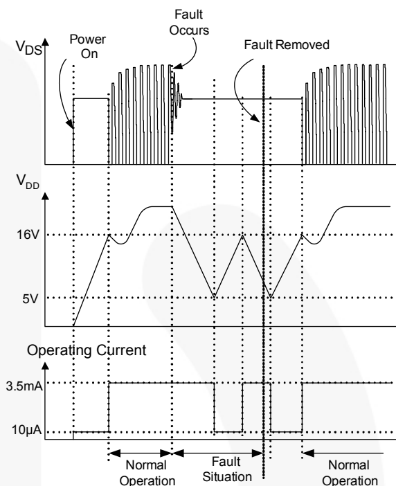
Figure 30. Auto-Restart Operation
