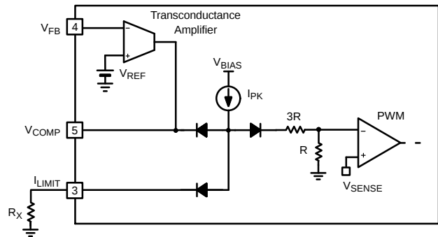
Figure 30. Current Limit Adjustment
