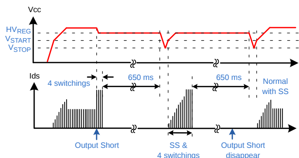
Figure 24. AOCP Waveform
