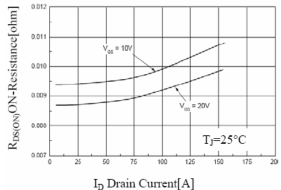
ON-Resistance Variation
