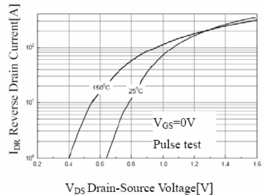
Body Diode Characteristics
