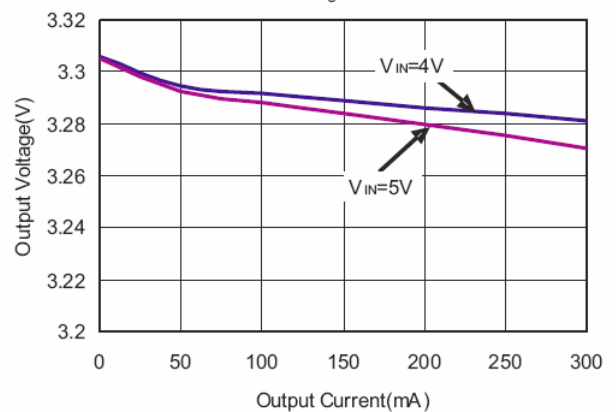
V_o = 3.3\text{V}
