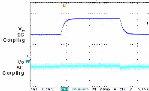
V_o=1.5V, V_{in}=2V to 3.3V, I_o=1mA
