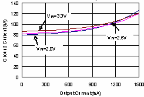
6. Ground Current vs Output Current
